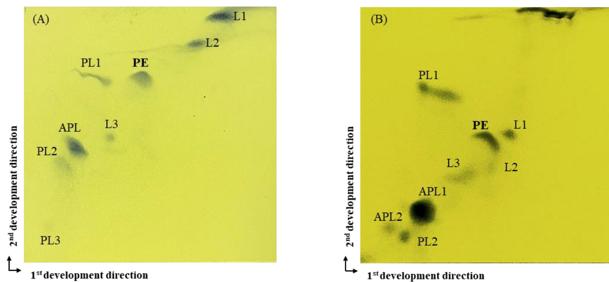
Fig. S4. Two-dimensional thin-layer chromatograms on the silica plates of total lipids of strains (A) KFT8 T and (B) CG01 T . Components were detected by spraying reagents with 5% ethanolic molybdotophosphoric acid.
