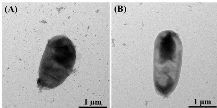
Fig. S2. Transmission electron micrographs of negatively stained (using 2% uranyl acetate) cells showing the general morphologies of strains D3-12 T (A) and G2-2 T (B) grown on marine agar at 30°C for 2 days.
