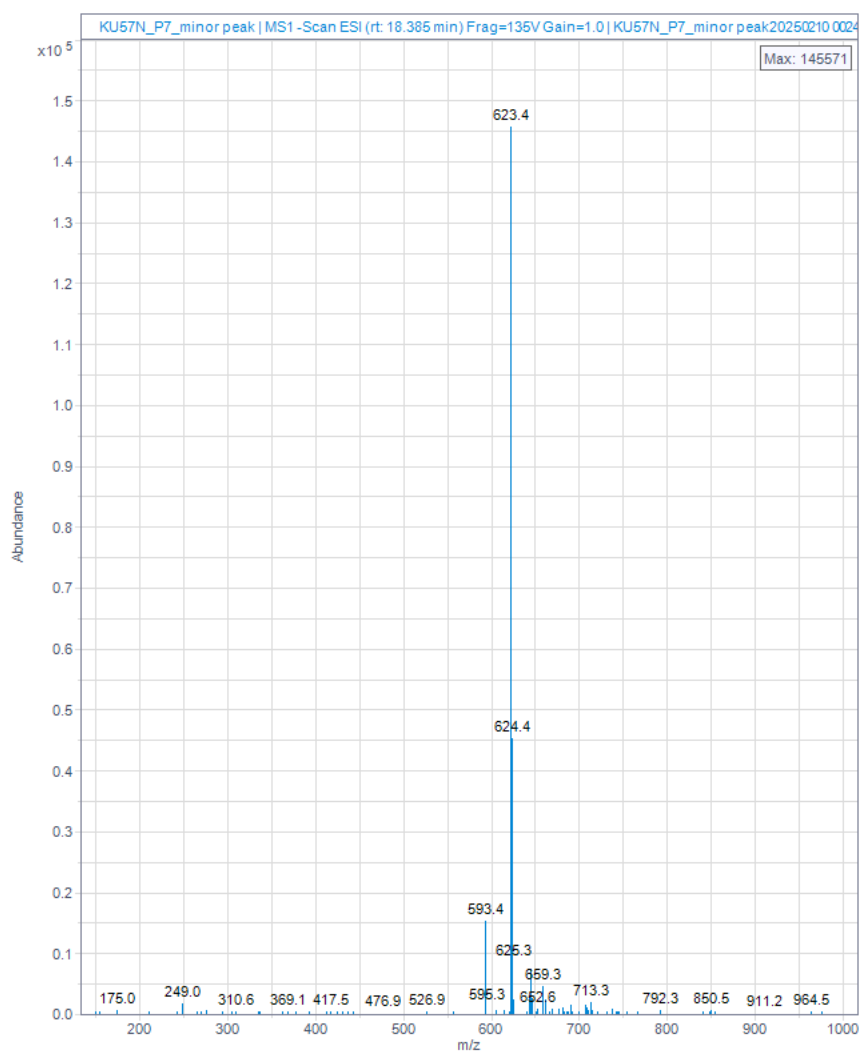
67 Fig. S14. LC-MS analysis of 4 .
