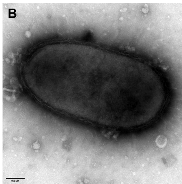
Fig. S1. Transmission electron micrographs of cells of strains IMCC43871 T (A), IMCC45206 T (B) after negative staining with 0.5% (w/v) uranyl acetate. Cells were grown on marine agar at 25°C for 7 days. Bar, 0.2 \mu m.
