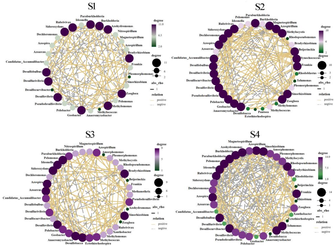
Fig. S3. Correlation network of dominant nitrogen-fixing microorganisms in rice root zone soil under CK treatment. A connection represents a strong ( |r| = 1 ) and significant ( p < 0.05 ) correlation between genera.
