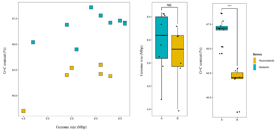
Fig. S6. Scatter and box plots for comparison of genome size (Mbp) and G + C content (%) between the genera Paraniabella and Niabella . Statistical significance was assessed using a t-test (NS, not significant; *** p < 0.001 ).
