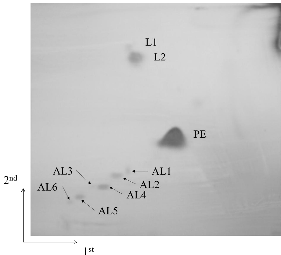
Fig. S9. Two-dimensional thin-layer chromatography of the polar lipids of strain CJ426 T . First dimension, chloroform/methanol/water (65:25:4); second dimension, chloroform/methanol/acetic acid/water (80:12:15:4). Abbreviations: PE, phosphatidylethanolamine; AL, amino lipid; L, unidentified lipid.
