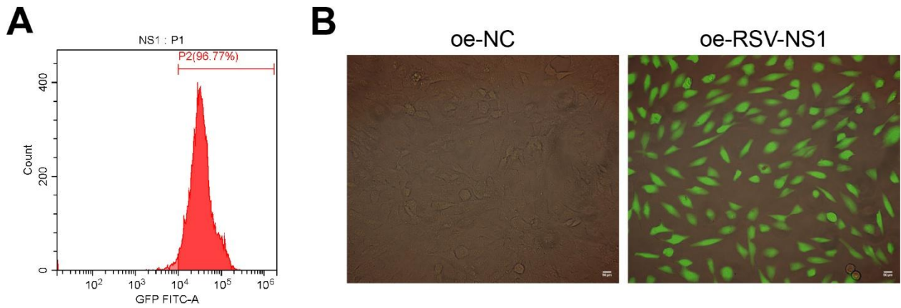
Fig. S2. Sorting and validation of NS1-positive Beas-2B cells. (A) Specific sorting of NS1-positive (NS1 + ) cell populations based on fluorescence signals using flow cytometry. (B) Immunofluorescence staining validation of NS1-positive cells. Scale bar = 50 \mu m.
